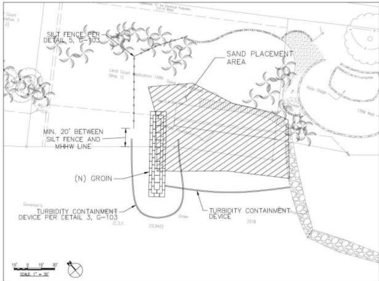
Attachment – Figure 1 Plan View of the Proposed Groin and Sand Placement Area DA File No. POH-2018-00220
